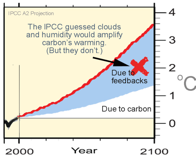
Theoretical warming due to carbon is only 35% of the total warming in projections; feedbacks (mostly humidity and clouds) amount to 65% of the warming.
